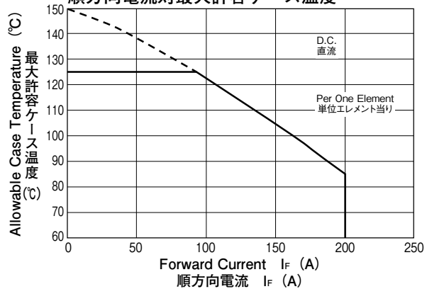
Forward Current vs. Allowable Case Temperature
