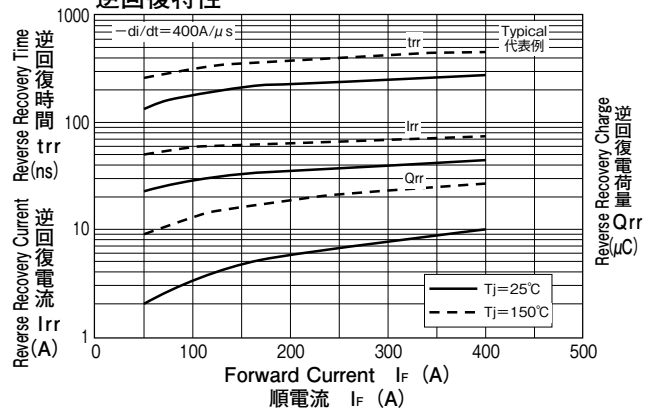
Reverse Characteristics
