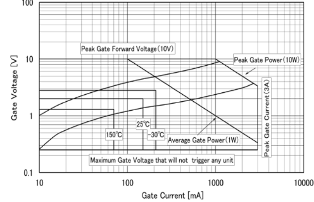
Gate Characteristics
