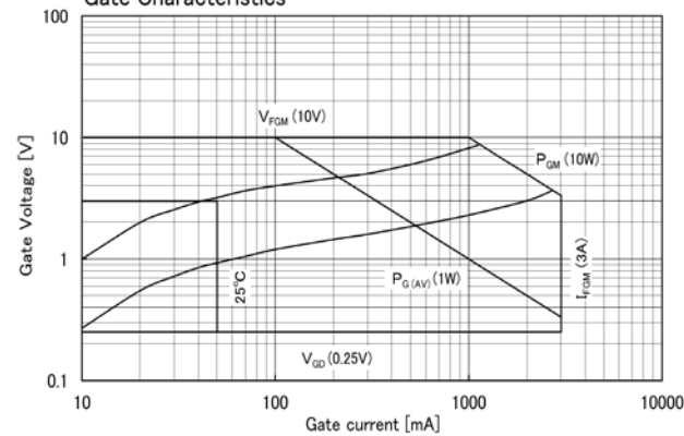
Gate Characteristics
