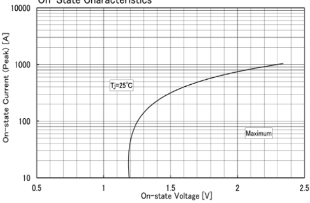
On-State Characteristics
